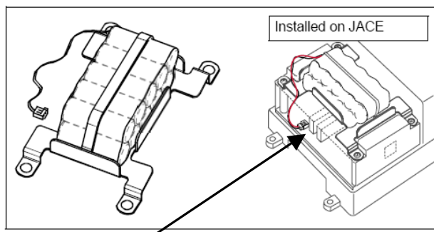
Figure 1 NPB-BATT assembly.
